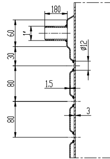
cooling jacket
